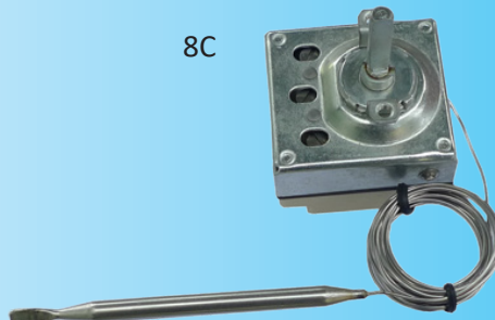
3 pole bulb and capillary thermostat, temperature ranges up to 320°C
